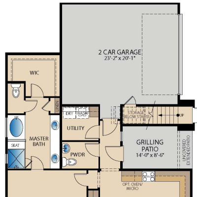
OPT. ADU - FIRST FLOOR
