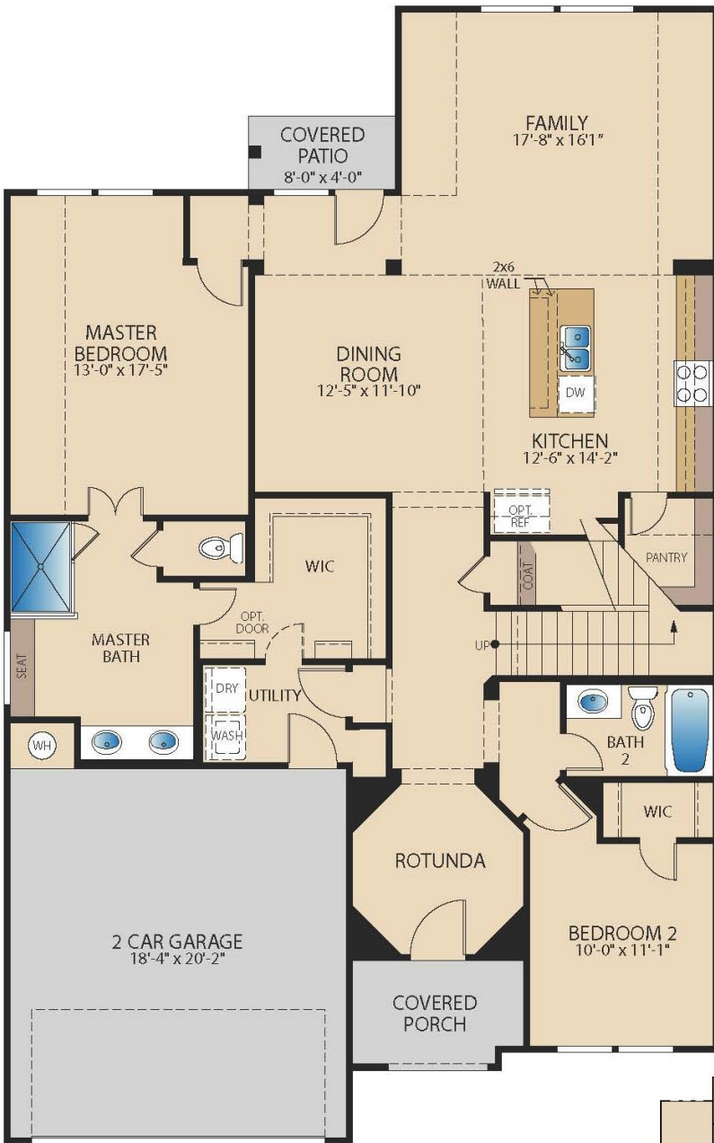
FIRST FLOOR
