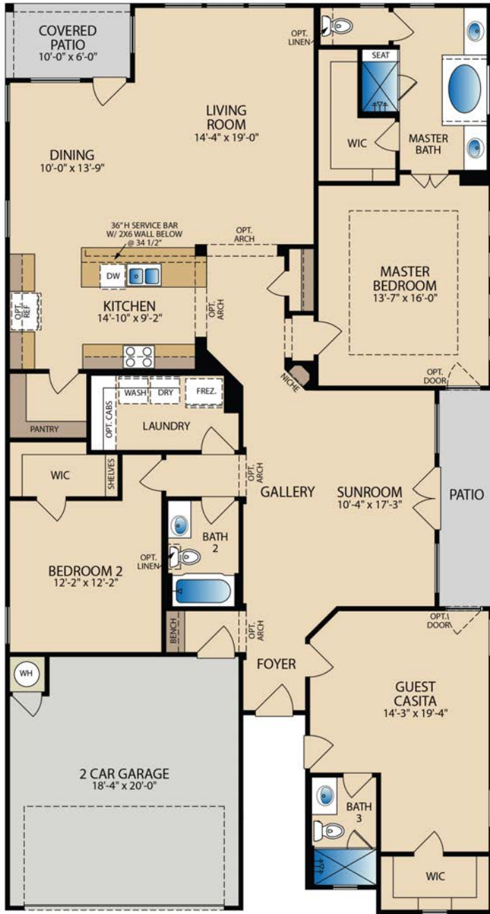
FLOOR PLAN
