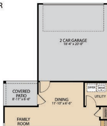
OPT. FIRST FLOOR PLAN WITH ATTACHED GARAGE
