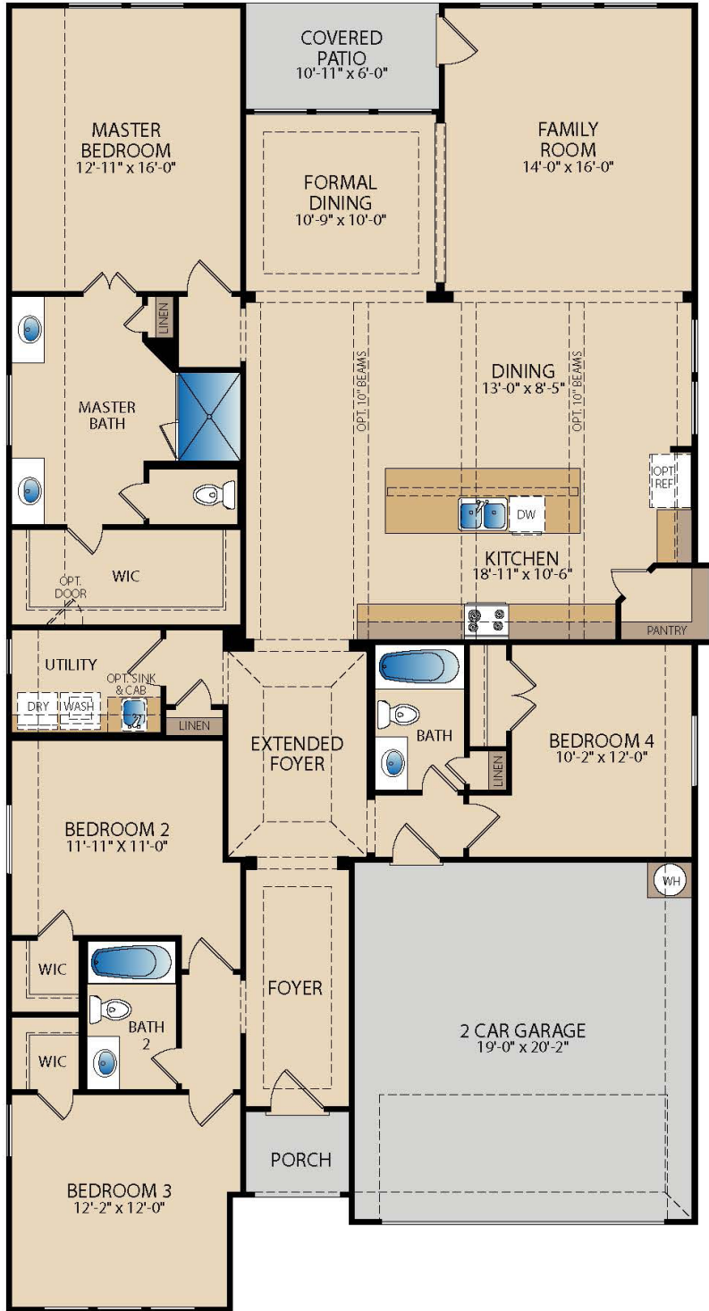
FIRST FLOOR
