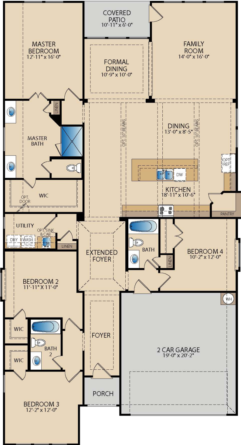
FIRST FLOOR
