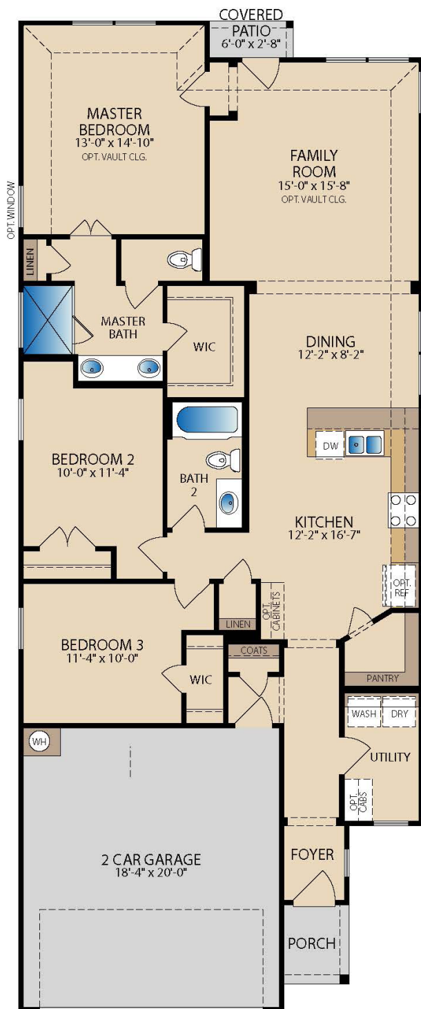
FLOOR PLAN
