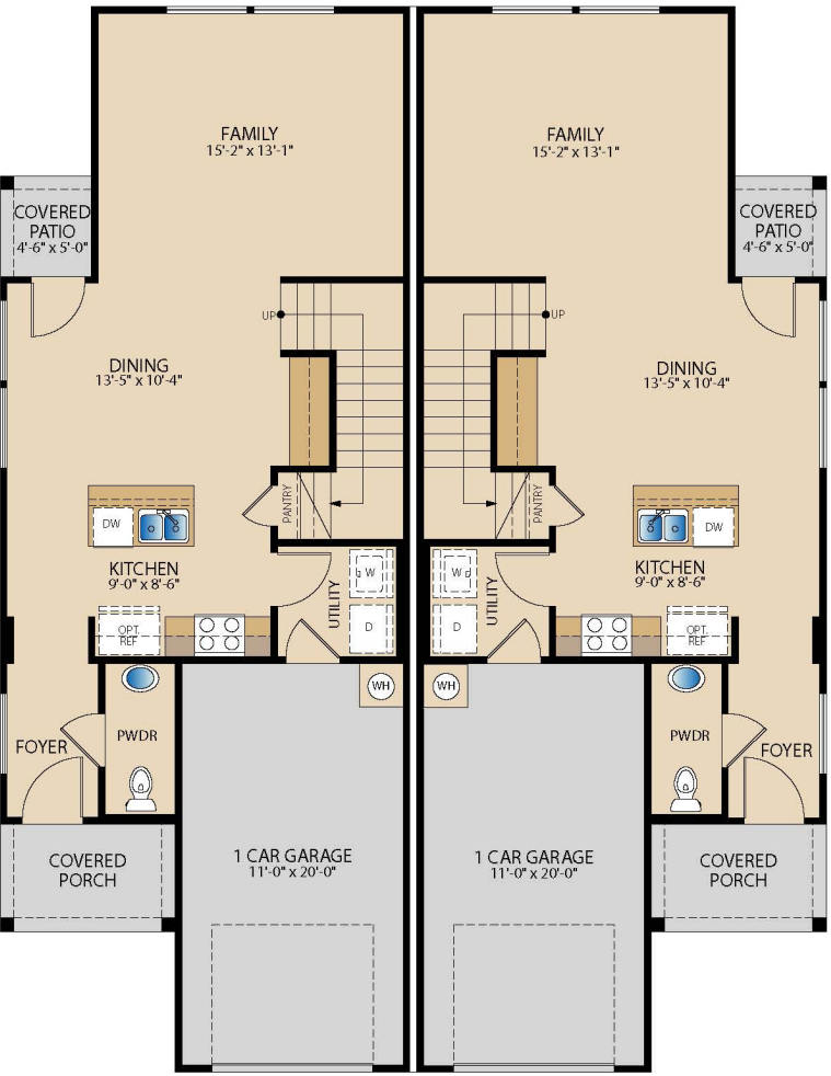
UNIT 1 UNIT 2 FIRST FLOOR
