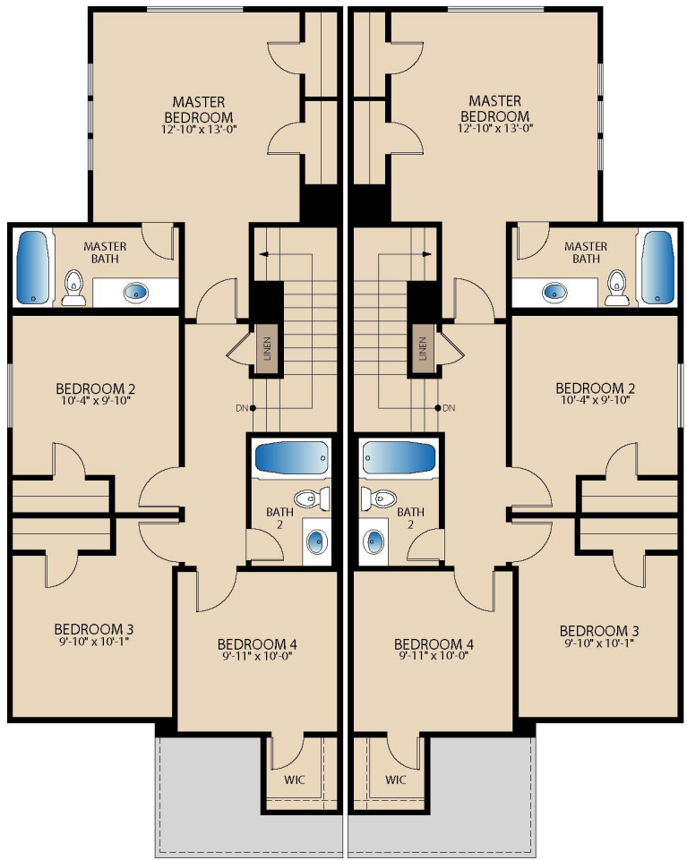
UNIT 1 UNIT 2 SECOND FLOOR
