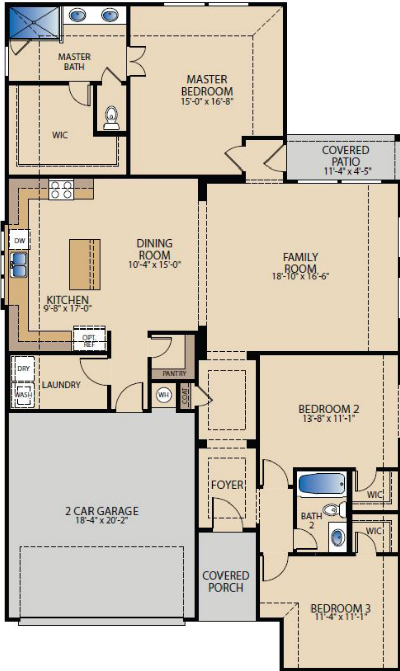
FLOOR PLAN
