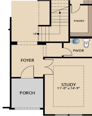
OPT. STUDY W/ POWDER 4 AT BEDROOM 2
