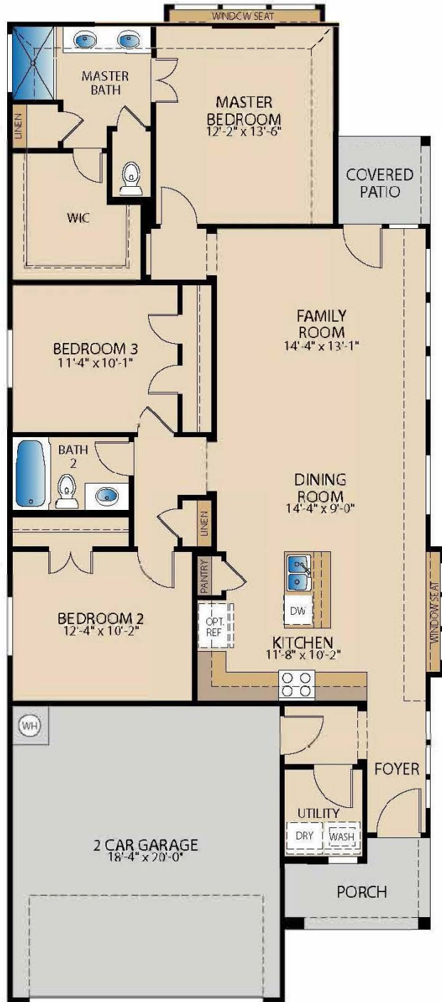
FIRST FLOOR
