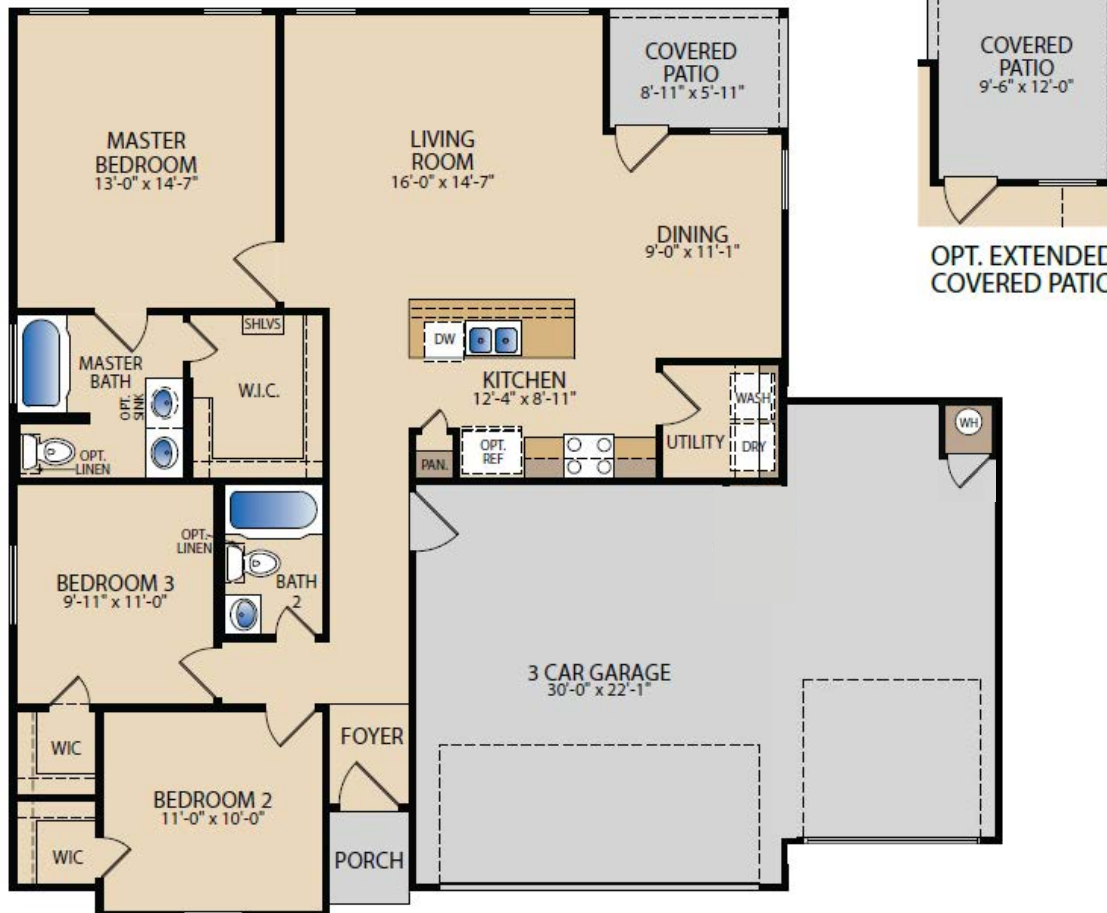
FIRST FLOOR
