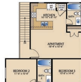
SECOND FLOOR PLAN W/OPT. APARTMENT ABOVE ATTACHED GARAGE
