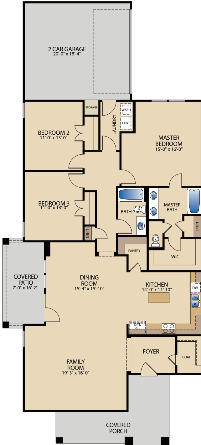
FLOOR PLAN
