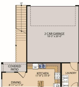
FIRST FLOOR PLAN W/OPT. APARTMENT ABOVE ATTACHED GARAGE
