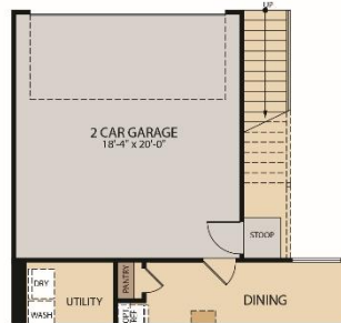
FIRST FLOOR W/ OPT. APARTMENT ABOVE ATTACHED GARAGE
