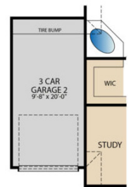
OPT. 3 CAR GARAGE 2
