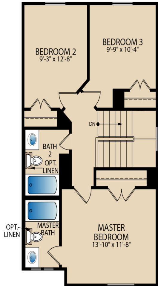
SECOND FLOOR
